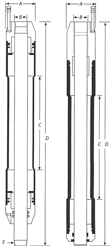
Standard Inflatable Packers
